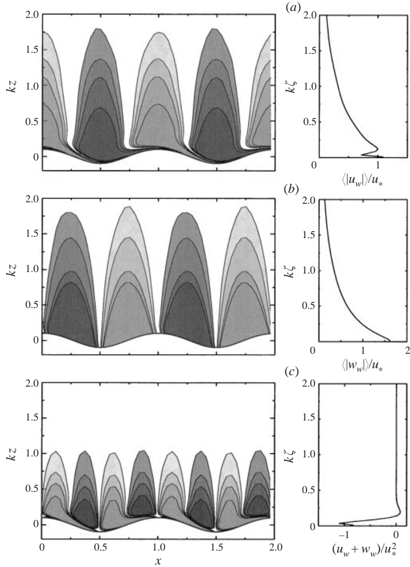
FIGURE 20. As figure 17 but for case (c/u_*, ak) = (22.7, 0.1) : (a) u_w , contours (\pm 0.2, \pm 0.3, \pm 0.4, \pm 0.6) ; (b) w_w , with contour values (\pm 0.2, \pm 0.3, \pm 0.5, \pm 0.6) ; (c) flux u_w w_w , contour values (\pm 0.1, \pm 0.2, \pm 0.3, \pm 0.5) .
